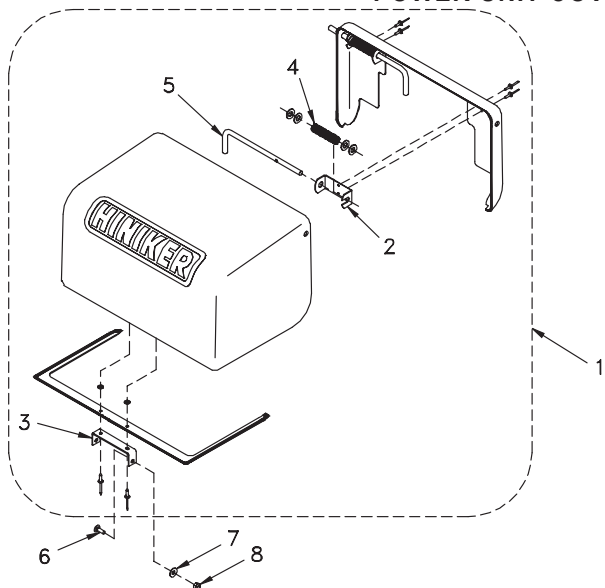
PLASTIC COVER ASSEMBLY
