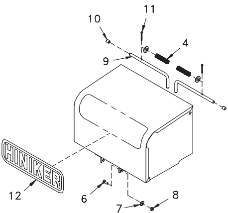
STEEL COVER ASSEMBLY
