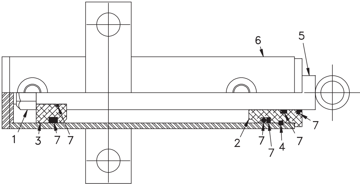
25010815 Hydraulic Cylinder
