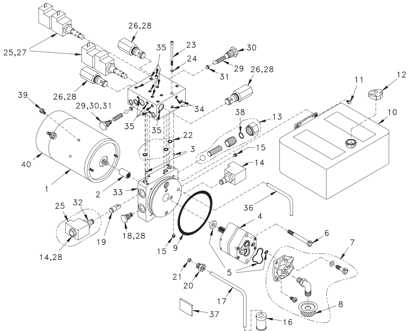
25010928 Power Unit
